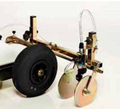
The iGO can have the spray head in front or to the side using a side arm.
